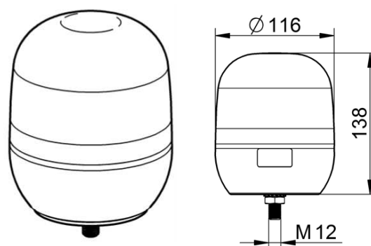
EUROROT LED P
