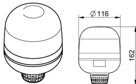
EUROROT LED A
