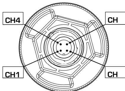
M12 Connector versions
